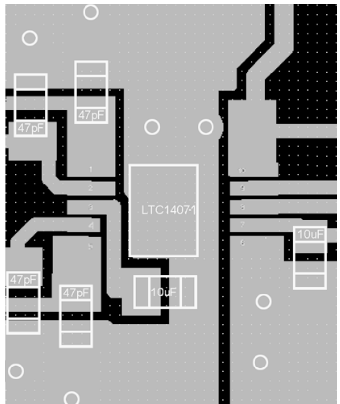
Figure 7. Recommended Layout
