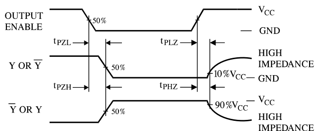
Figure 4. Switching Waveforms
