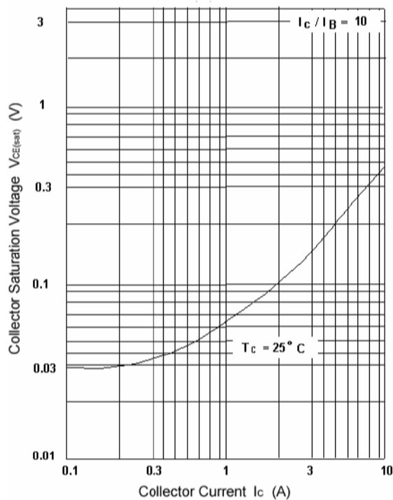
Fig.5 Collector-Emmitter Saturation Voltage
