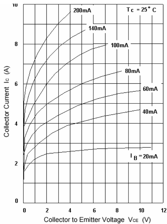
Fig.3 Static Characteristic
