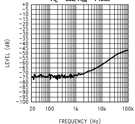
Power Supply Rejection Ratio (PSRR) at A_V = 2 V_{DD} = 5V , V_{ripple} = 200mvp-p R_L = 8\Omega , R_{IN} = \text{Float}
