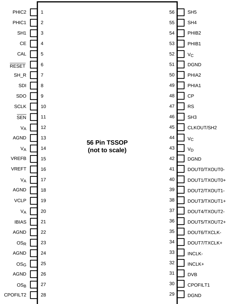
56-Pin TSSOP Package DGG Top View
