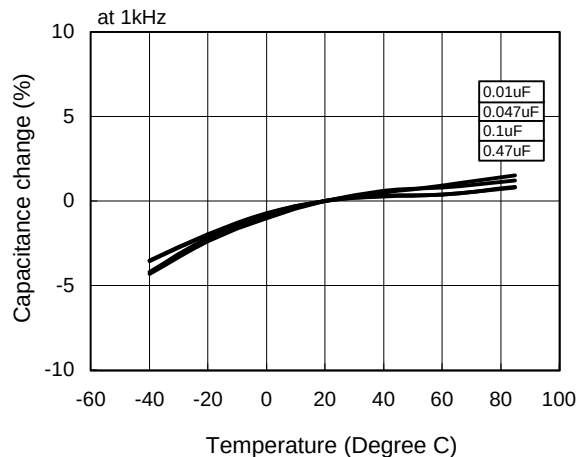
Temperature Characteristics
