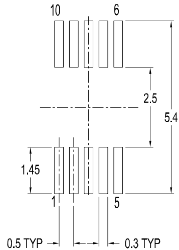
LAND PATTERN RECOMENDATION
