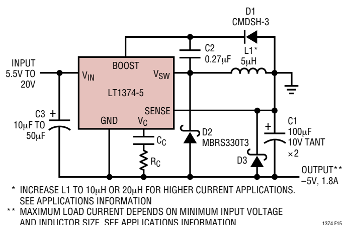
Figure 15. Positive-to-Negative Converter
