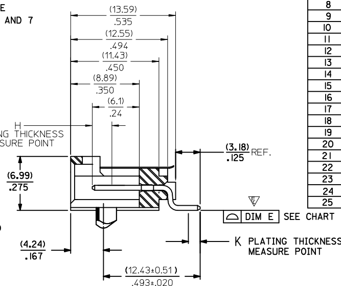
SECTION F-F
