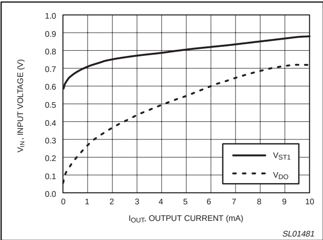
Figure 17. Output current versus starting voltage.
