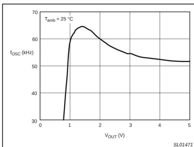
Figure 8. Oscillator frequency versus V_{OUT} .
