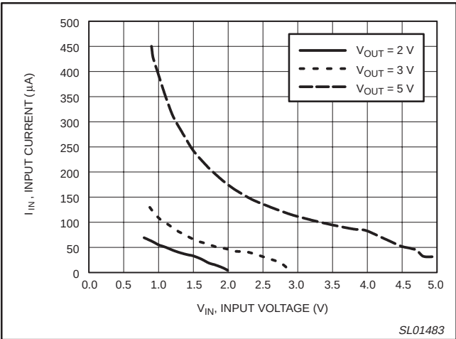
Figure 19. Input voltage versus supply current.
