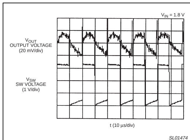
Figure 11. Ripple voltage at I_{OUT} = 60 mA .
