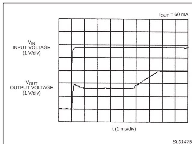
Figure 12. Start-up characteristic V_{IN} : 0 V \rightarrow 1.8 V .
