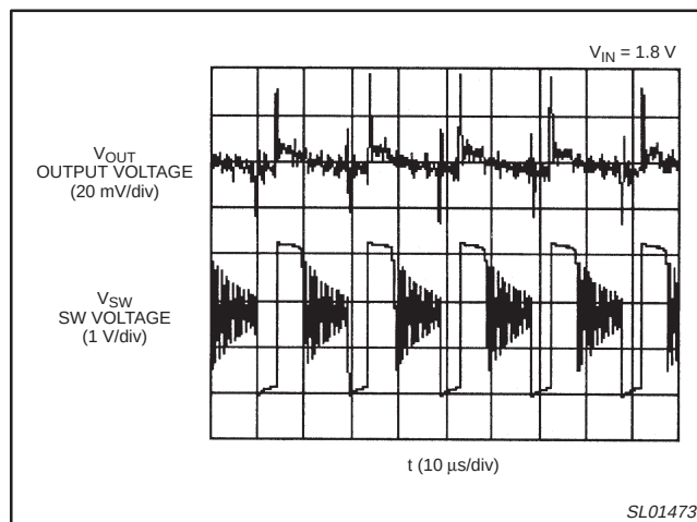
Figure 10. Ripple voltage at I_{OUT} = 10 mA .
