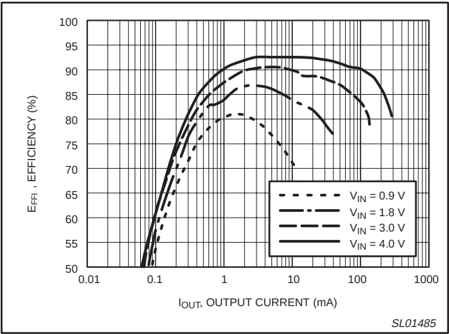
Figure 21. Output current versus efficiency (100 \mu H inductor).
