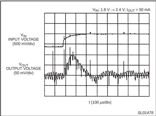
Figure 15. Input line regulation, increasing voltage.
