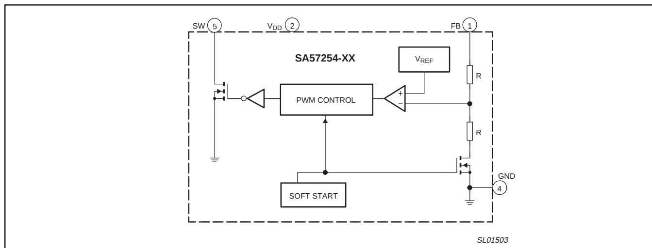
Figure 23. Functional diagram.
