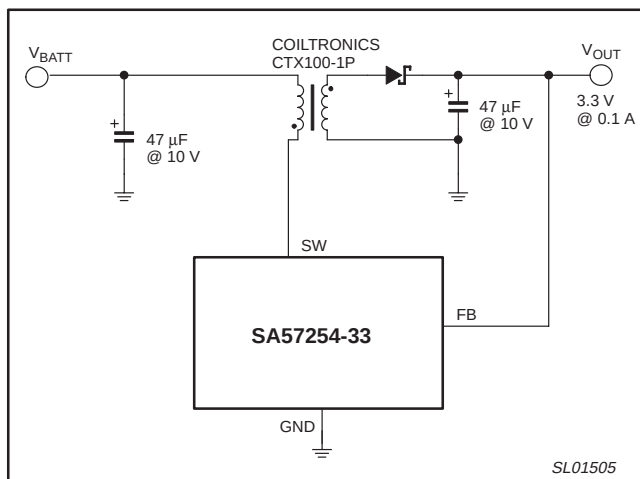
Figure 27. Flyback converter circuit.
