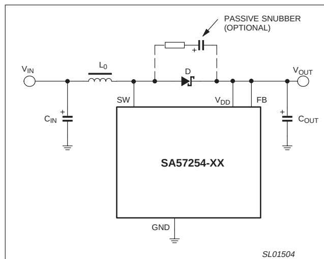
Figure 24. Boost converter.
