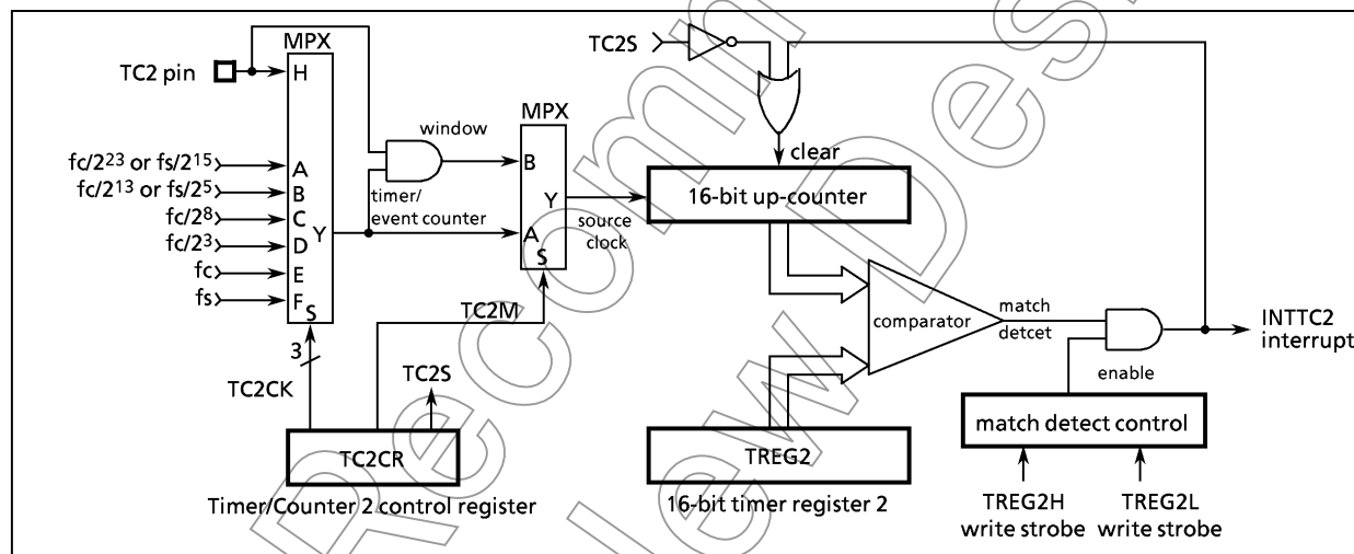
Figure 2-21. Timer/Counter 2 (TC2)
