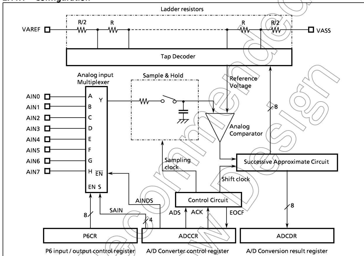
Figure 2-43. A/D Converter
