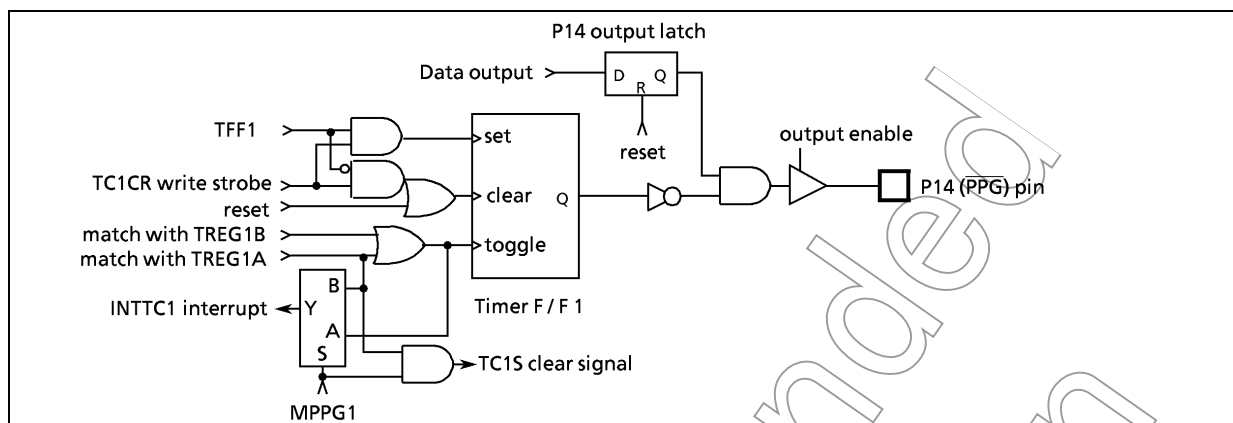
Figure 2-20. PPG Output
