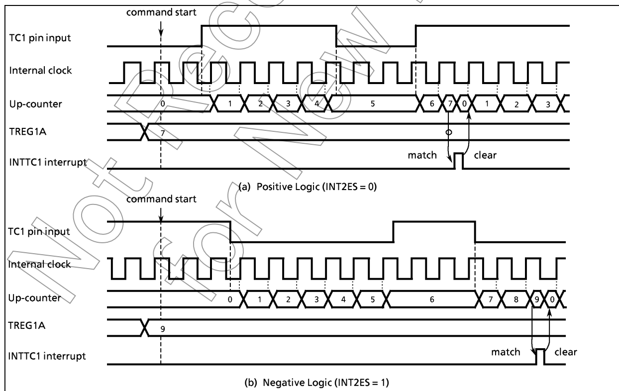
Figure 2-17. Window Mode Timing Chart
