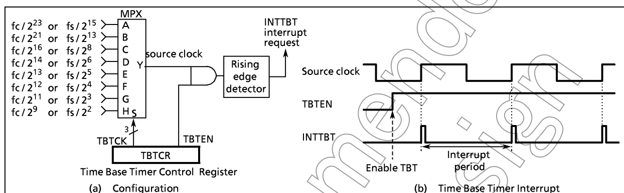
Figure 2-8. Time Base Timer
