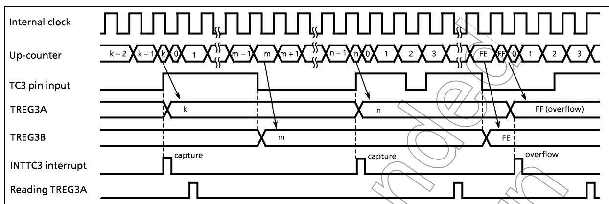
Figure 2-26. Timing Chart for Capture Mode (INT3ES = 0)
