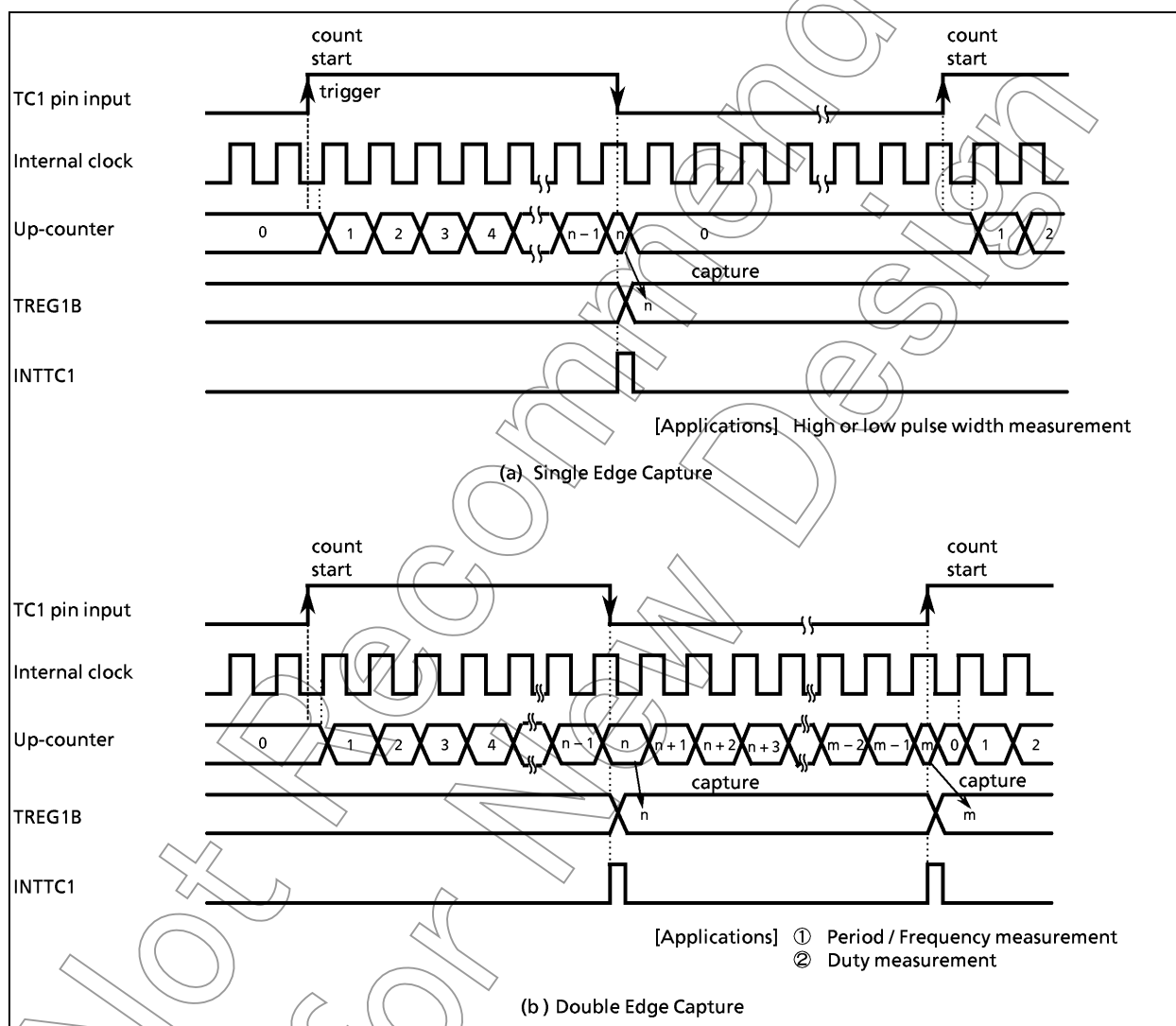
Figure 2-18. Pulse Width Measurement Mode Timing Chart
