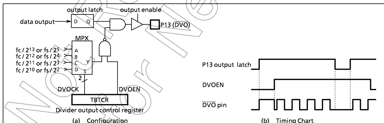
Figure 2-11. Divider Output
