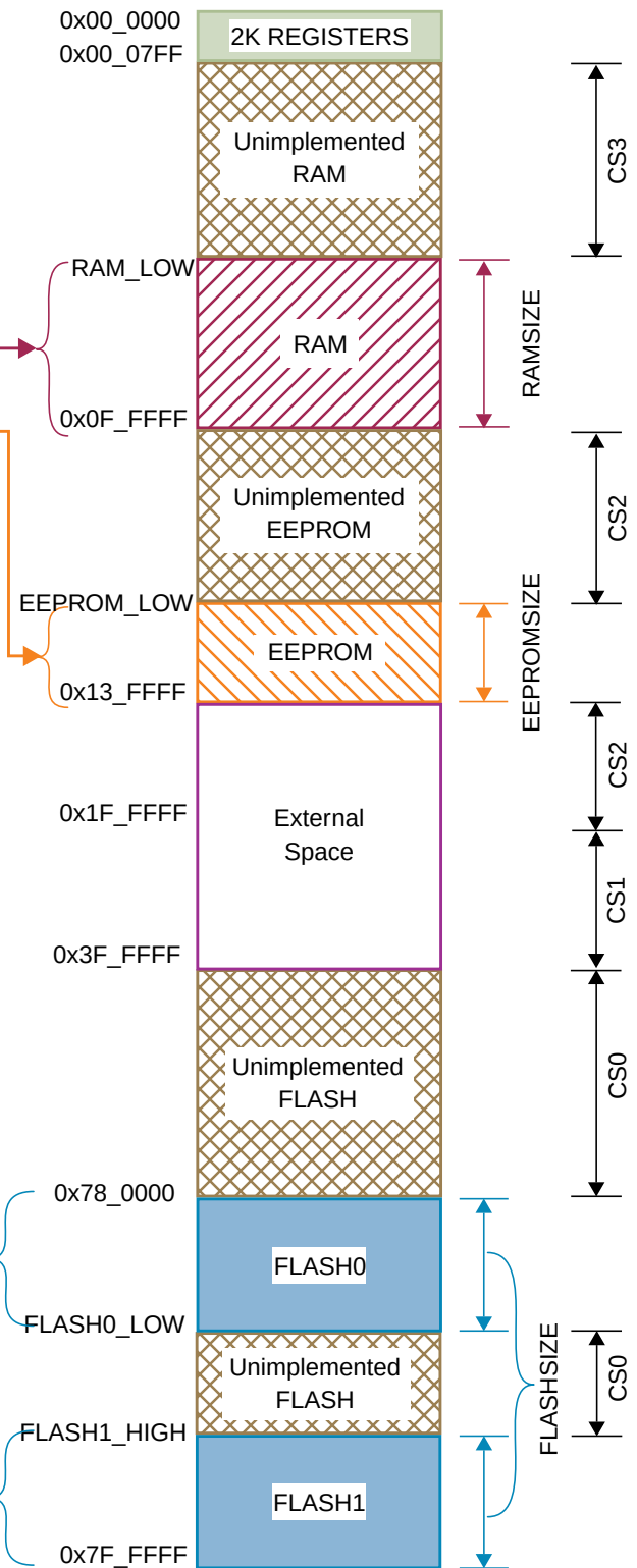
Figure 1-4. S12X CPU & BDM Global Address Mapping
