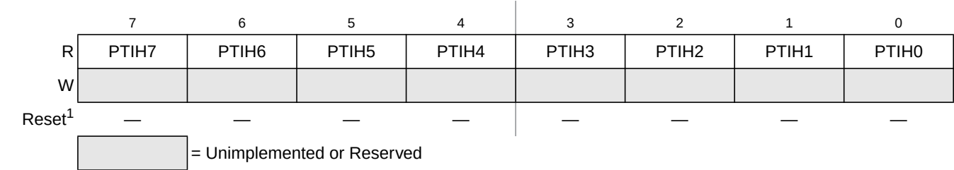
Figure 22-49. Port H Input Register (PTIH)
