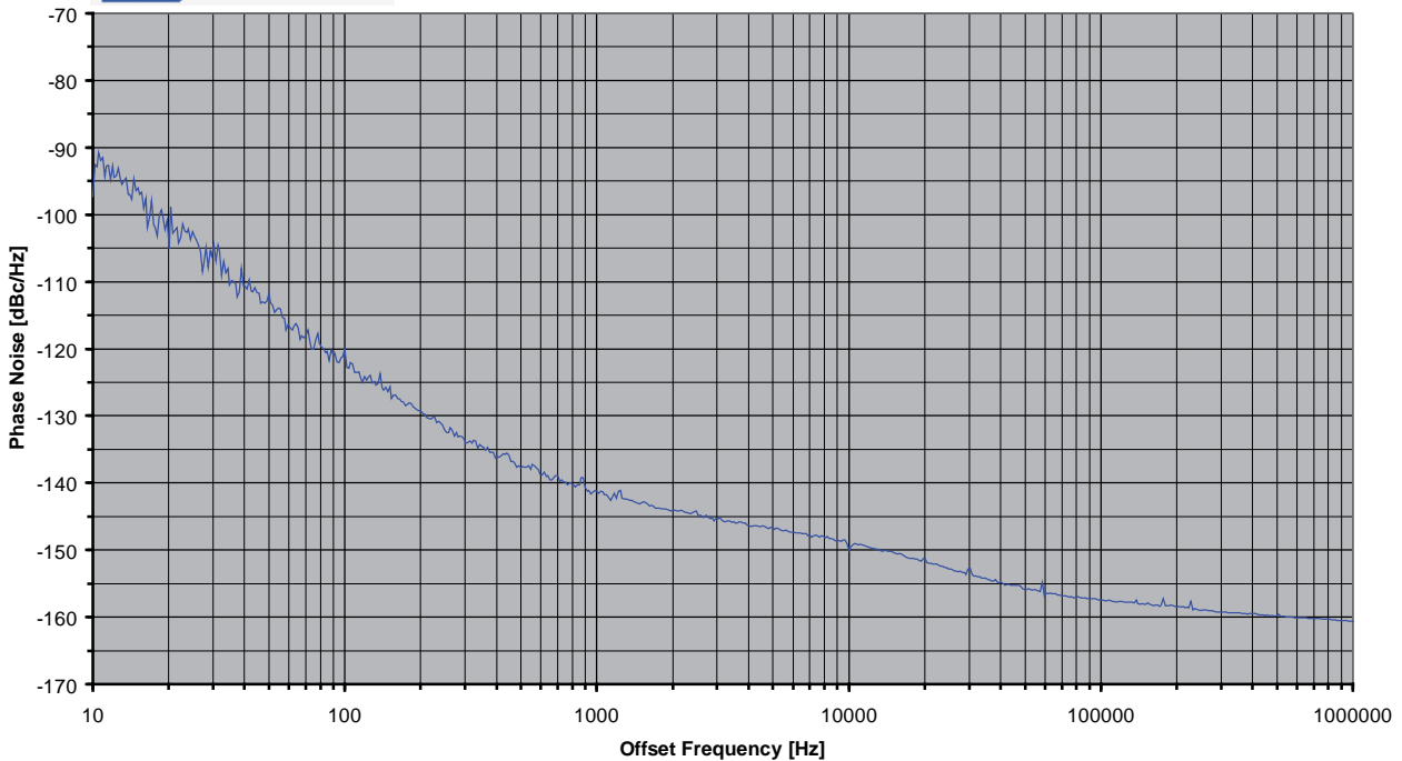
Typical Phasenoise: PX-508 @ 120MHz
