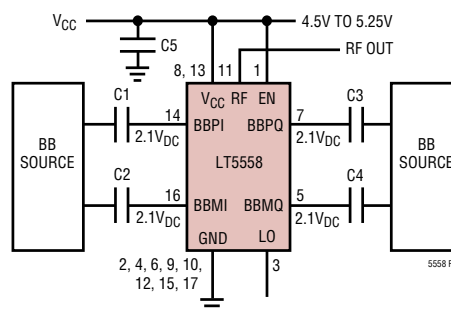
Figure 3. AC-Coupled Baseband Interface
