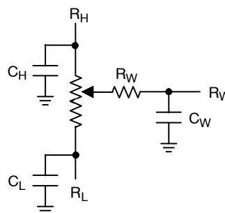
Figure 2. Potentiometer Equivalent Circuit
