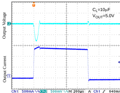
Figure 13. Load Transient
