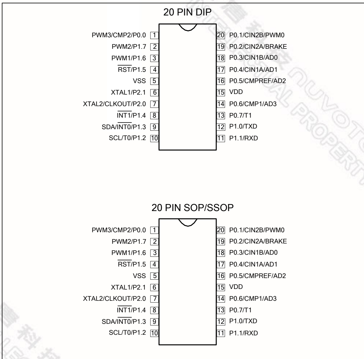
Figure 4-1: Pin Configuration
