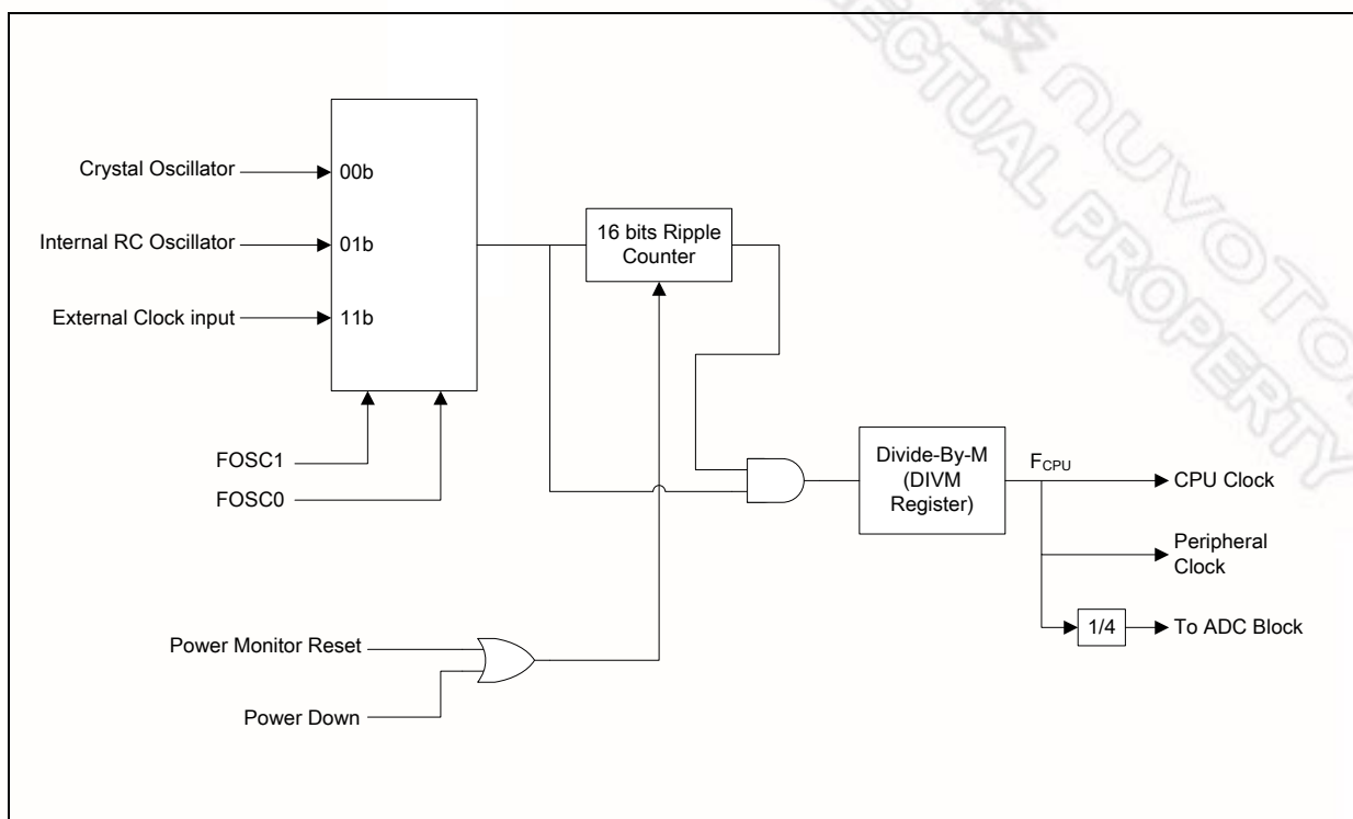
Figure 21-1: Oscillator
