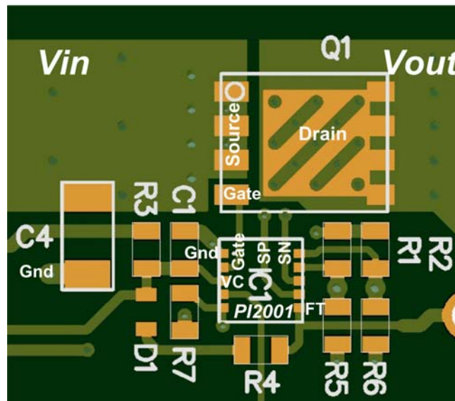
Figure 18: PI2001 and MOSFET layout recommendation
