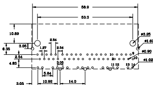
PCB LAYOUT - component side view
