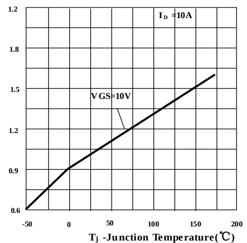
Figure.4 R_{DS(on)} -Junction Temperature
