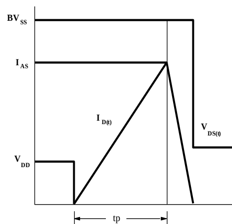
3) Unclamped Inductive Test Circuit & Waveforms
