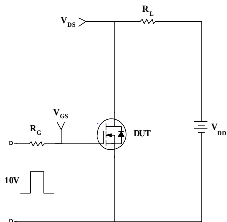
2) Switching Test Circuit & Waveforms
