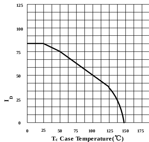
Figure.6 Drain Current VS Case Temperature
