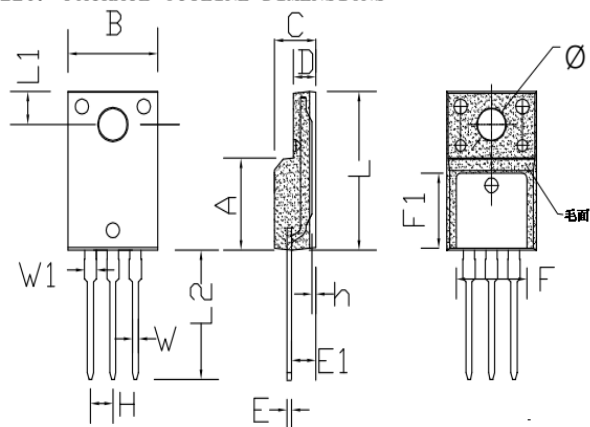
T0-220F PACKAGE OUTLINE DIMENSIONS
