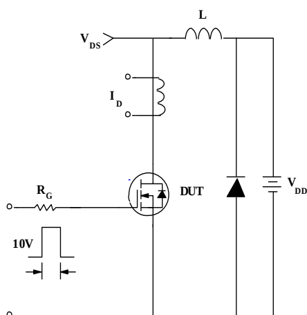
3) Unclamped Inductive Test Circuit & Waveforms
