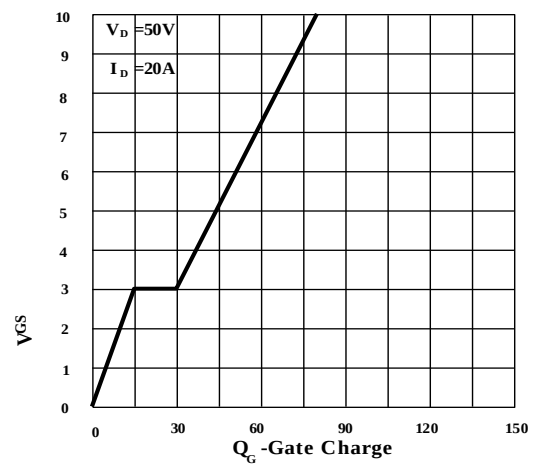
Figure.8 Gate Charge
