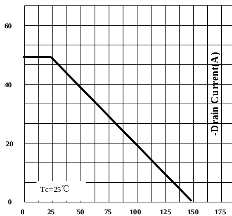
Figure.9 Power De-rating
