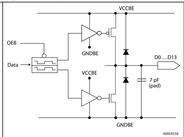
Figure 4. Output buffers
