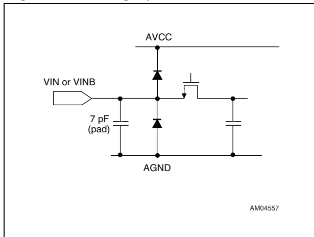
Figure 3. Analog inputs
