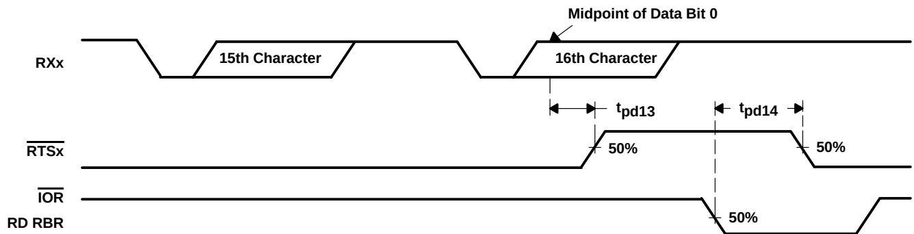
Figure 17. Auto-RTS Timing for RCV Threshold of 14 Waveforms
