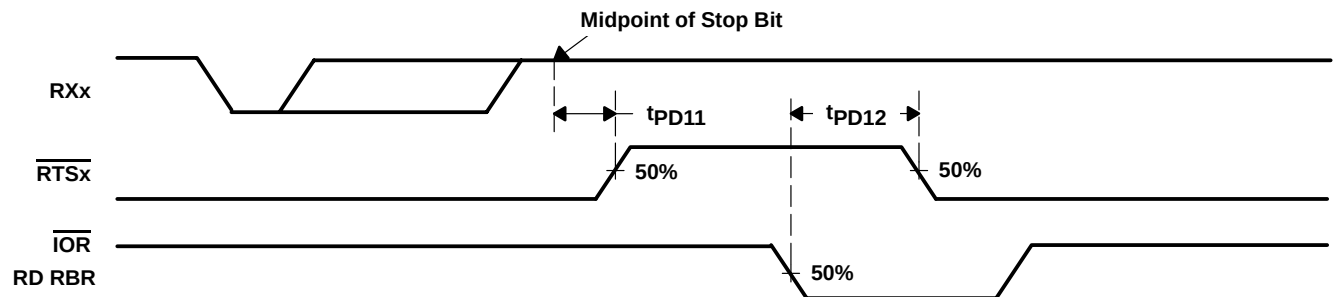
Figure 16. Auto-RTS Timing for RCV Threshold of 1, 4, or 8 Waveforms
