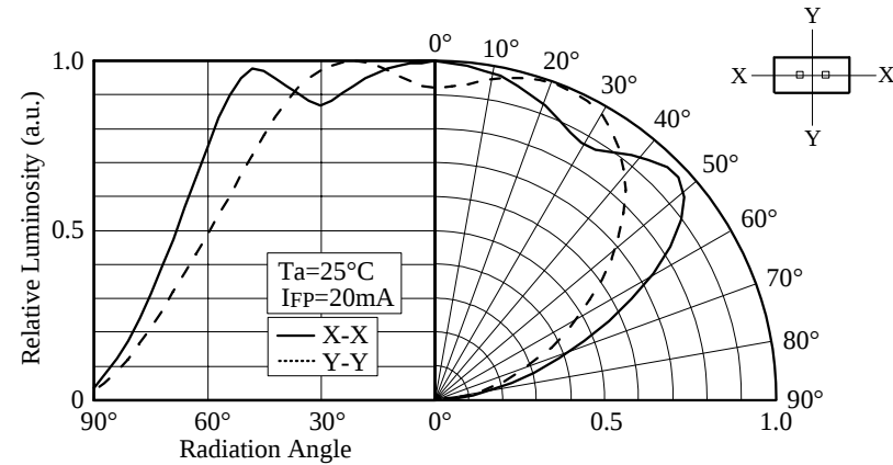
■ Directivity
