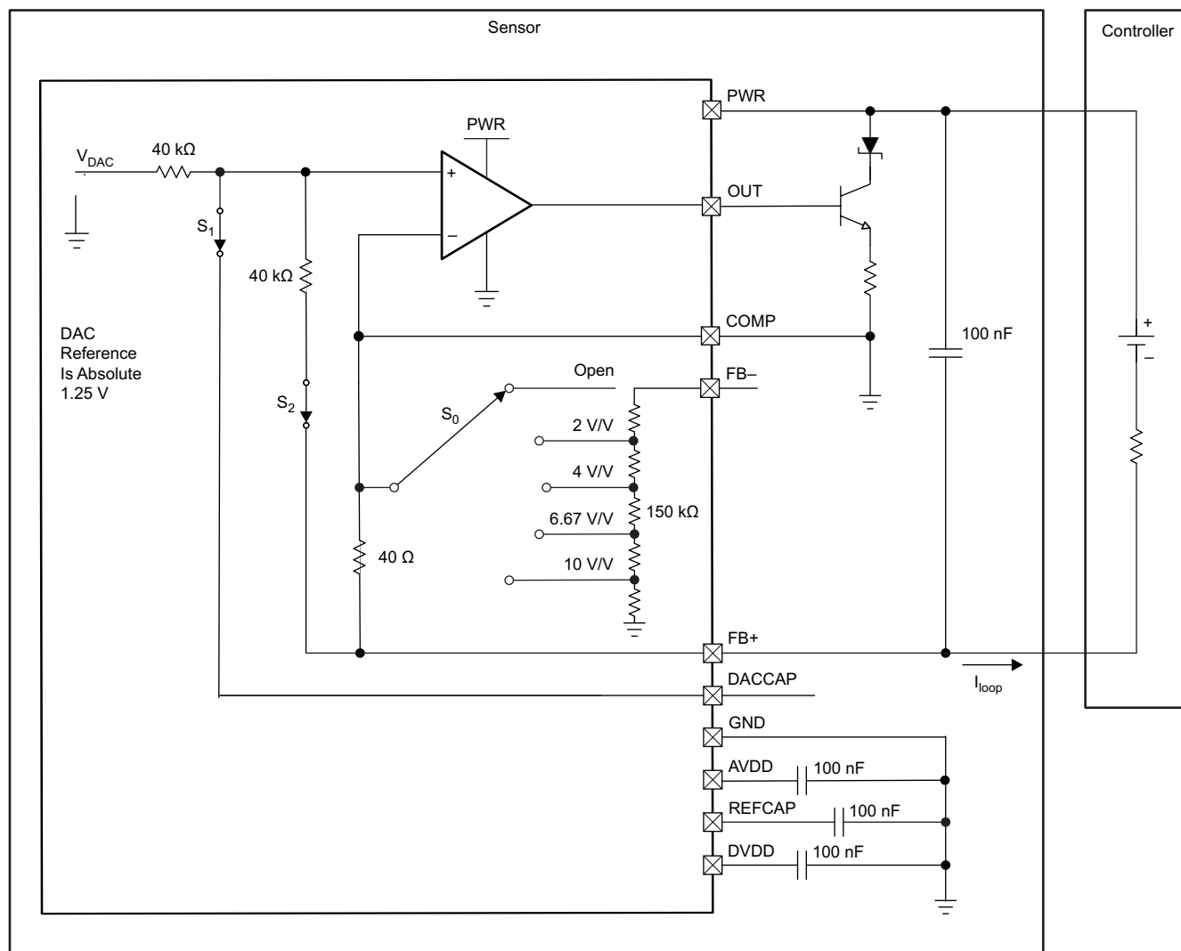
图 40. 4-mA to 20-mA Output With Internal Sense Resistor Diagram
