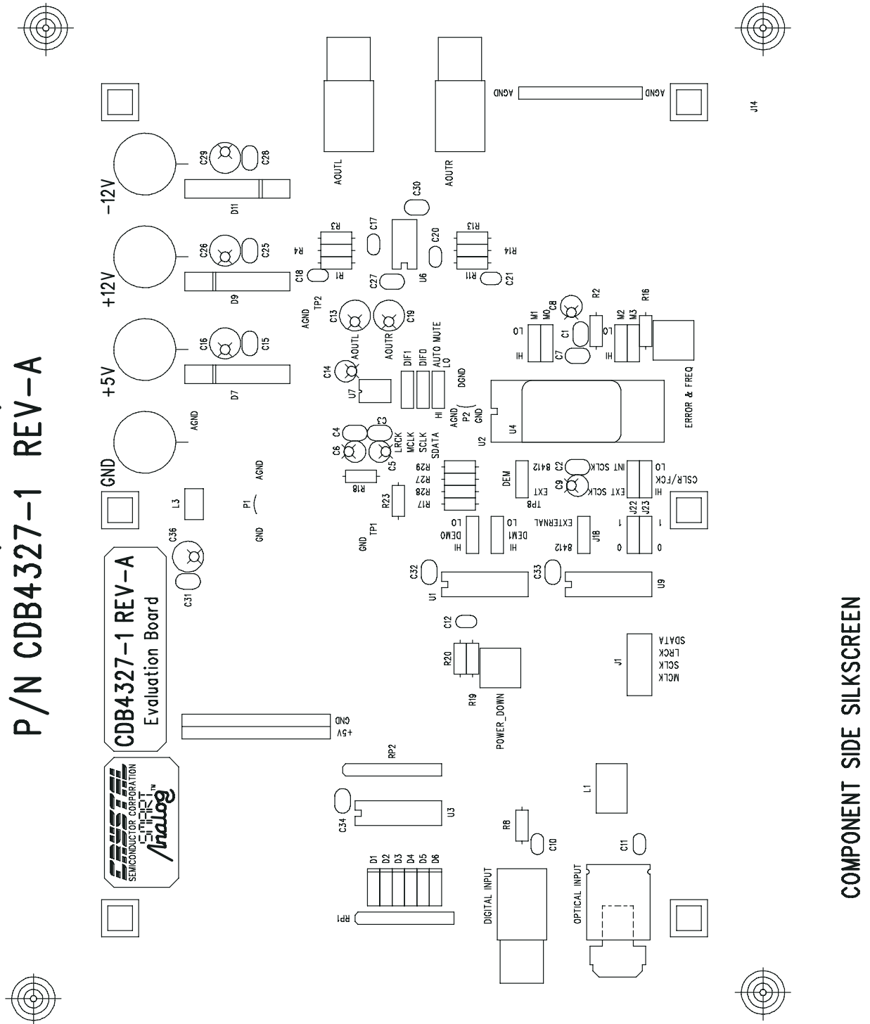
Figure 10. CDB4327 Component Side Silkscreen
