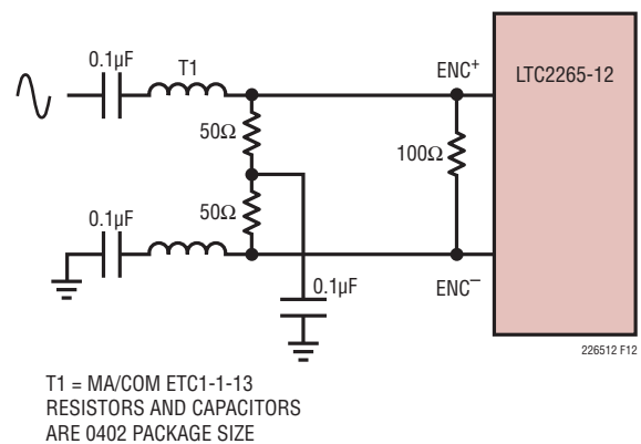
Figure 12. Sinusoidal Encode Drive
