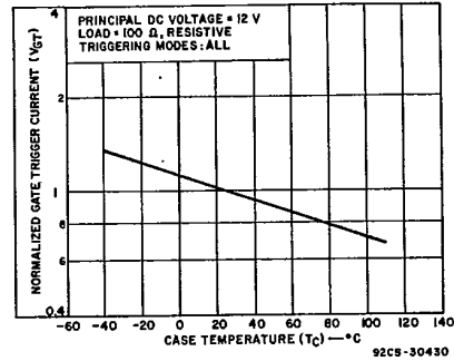
Fig. 8 - Normalized gate trigger voltage as a function of case temperature.
