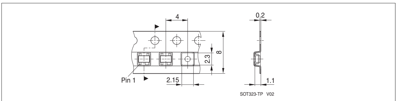
Figure 23 Tape Dimensions
