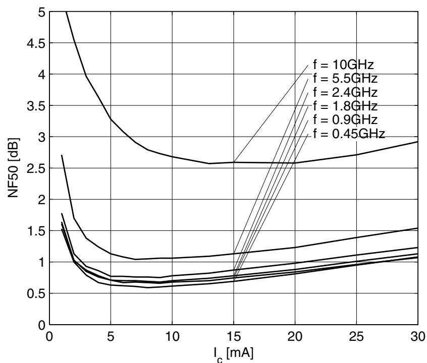
Figure 19 Noise Figure NF_{50} = f(I_c) , V_{CE} = 3\text{ V} , Z_S = 50\ \Omega , f = \text{Parameter in GHz}
