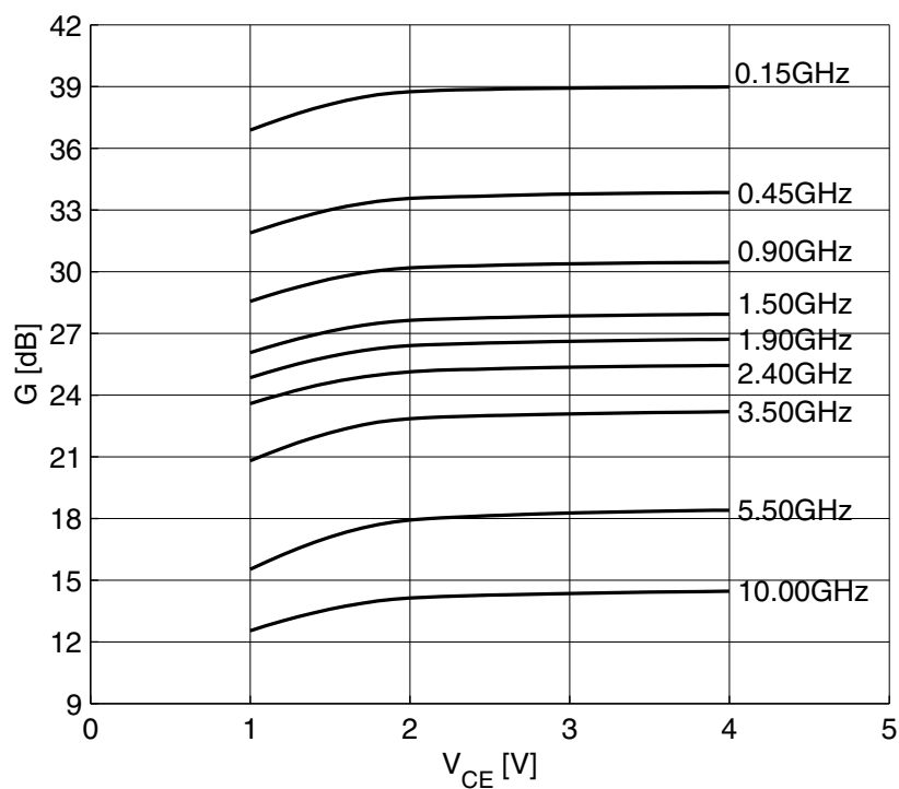
Figure 13 Maximum Power Gain G_{\max} = f(V_{CE}) , I_C = 25 \text{ mA} , f = \text{Parameter in GHz}
