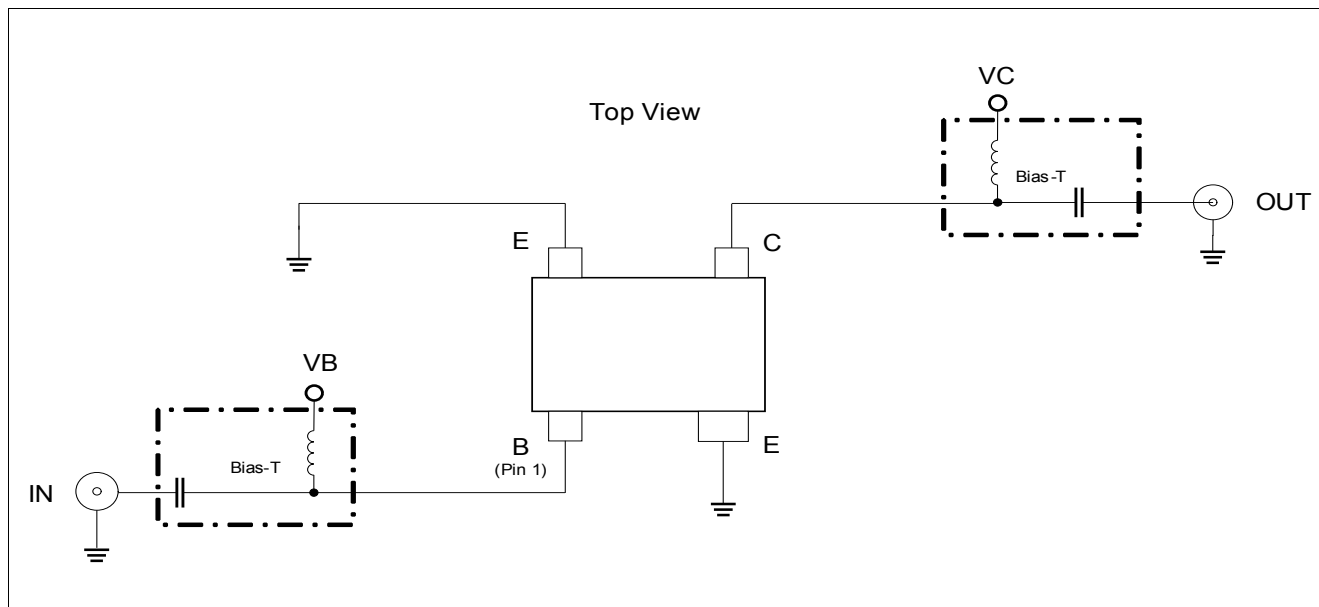
Figure 2 BFP740ESD Testing Circuit
