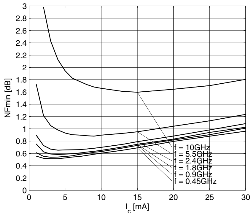
Figure 18 Noise Figure NF_{min} = f(I_c) , V_{CE} = 3\text{ V} , Z_S = Z_{opt} , f = \text{Parameter in GHz}
