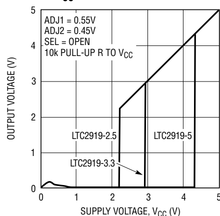
OUT1, OUT2, \overline{\text{RST}} Output Voltage vs V_{CC}
