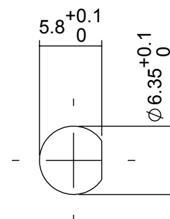
Mounting Hole
