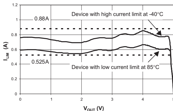
Figure 1: Current Limit Using 10.5kΩ.
