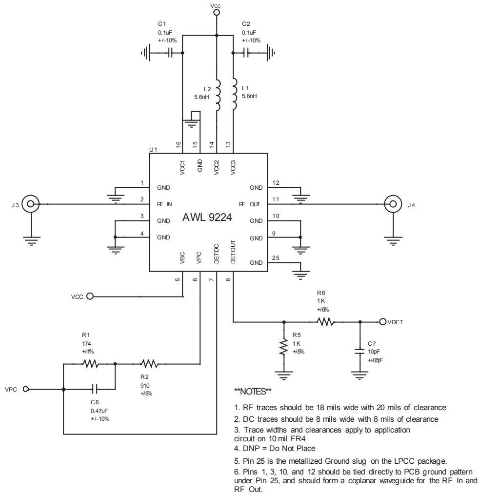
Figure 19: Application Circuit
