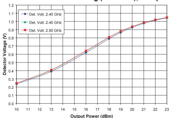
Figure 15: Detector Voltage vs. Output Power Across Frequency ( T_C = 25^\circ C , V_{CC} = +3.3V ) 802.11b Gaussian Filtering (BT = 0.45), 1 Mbps
