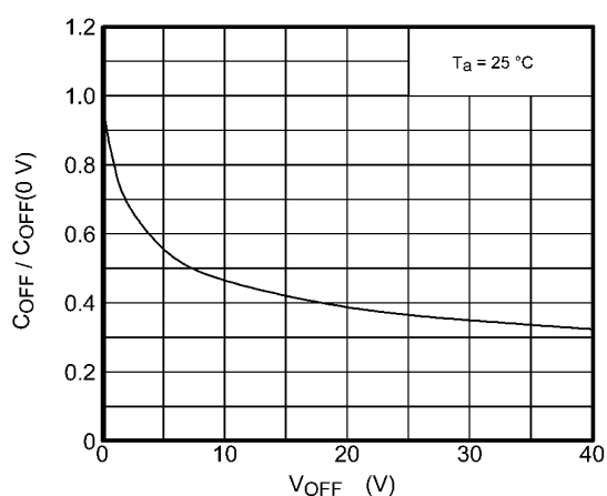
Fig. 12.1.10 C_{OFF}/C_{OFF}(0\text{ V}) - V_{OFF}
