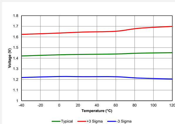
Figure 39-80. POR Rearm Voltage, VREGPM1 = 0, PIC18F26/45/46K40 only
