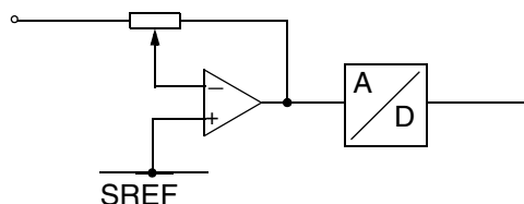
Fig. 5-9: Analog input pins MIC, MICBIAS, ADCL, ADCR
