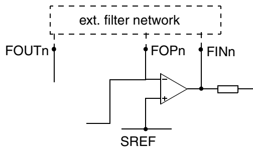
Fig. 5-4: Pins FINR, FOPR, FINL, FOPL
