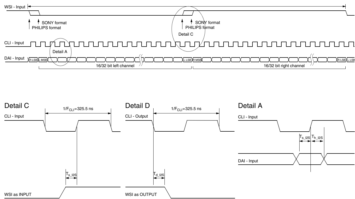
Fig. 5-21: Timing asynchronous I 2 S input
