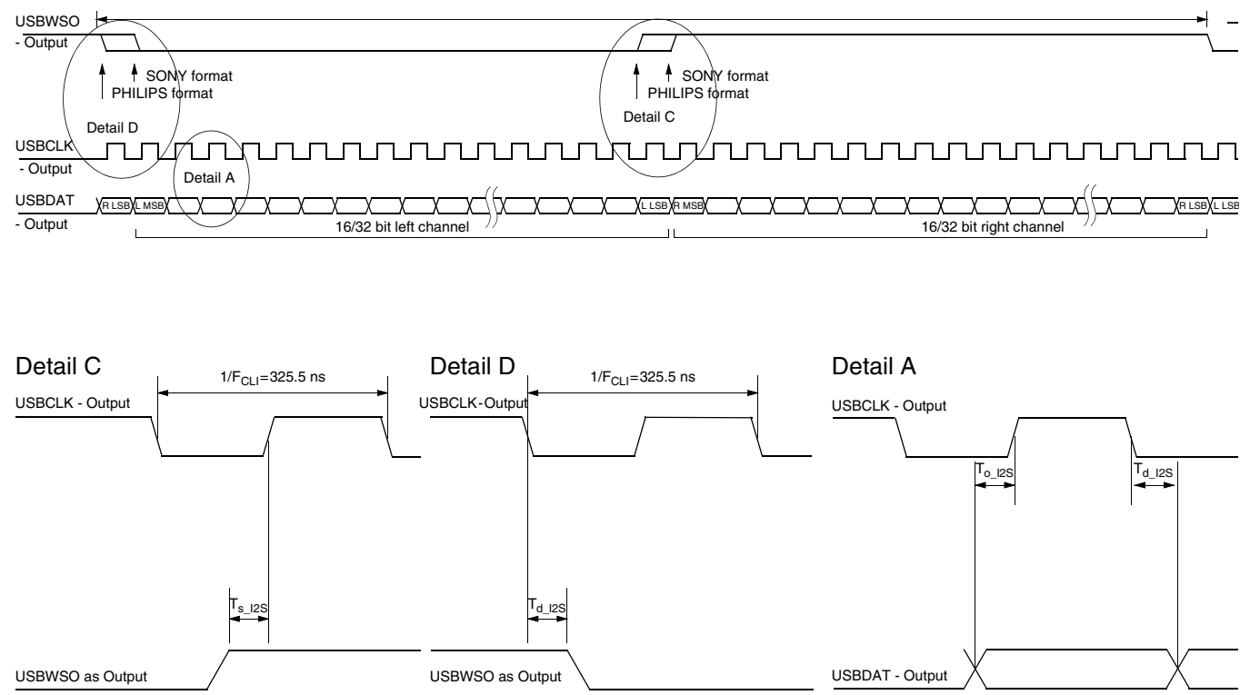
Fig. 5-22: Timing synchronous I 2 S output
