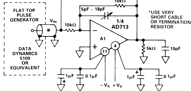
Figure 1. Settling Time Test Circuit
