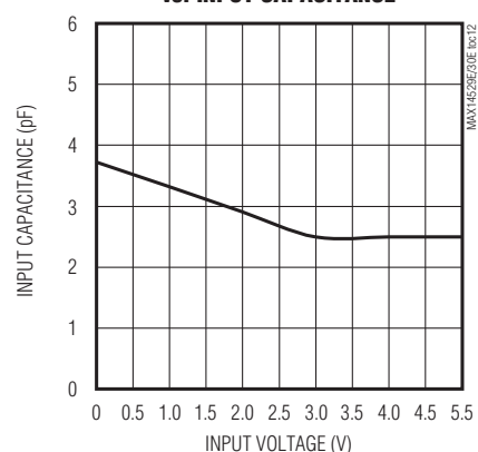
D+/D- INPUT VOLTAGE vs. INPUT CAPACITANCE
