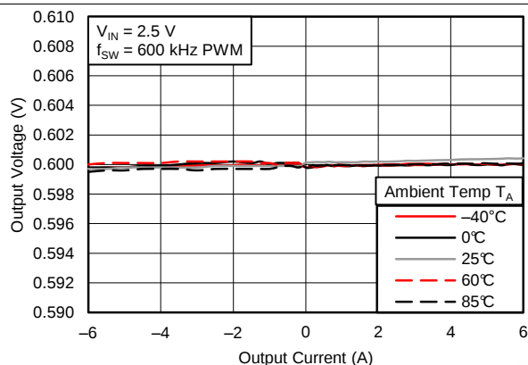
Figure 7. Load Regulation
