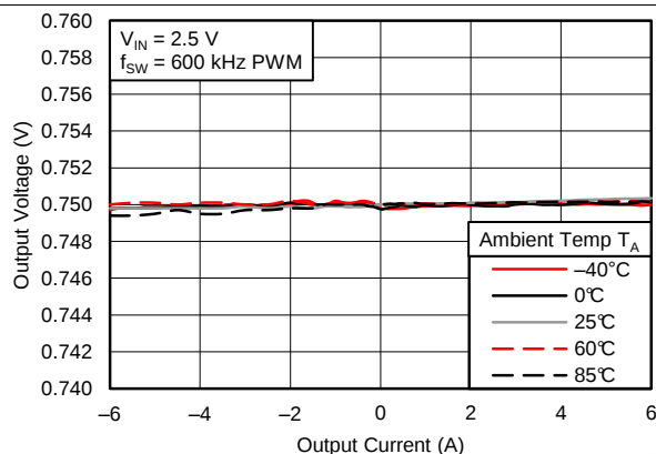
Figure 8. Load Regulation
