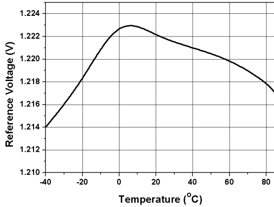
Fig. 7 V_{\text{REF}} vs. Temperature
