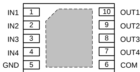
U-DFN3030-10
