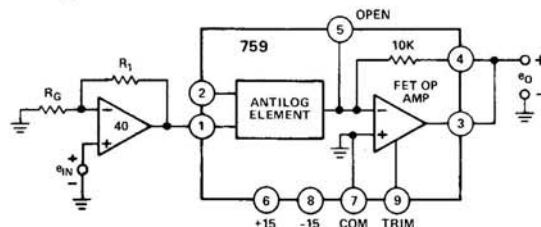
Figure 6. Method for Adjusting K < 2/3V
