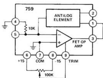
Figure 3. Trimming E_{OS} in Log Mode
