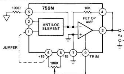
Figure 5. Trimming E_{OS} in Antilog Mode
