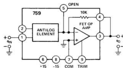
Figure 4. Functional Block Diagram
