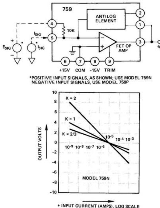
Figure 1. Functional Block Diagram and Transfer Function
