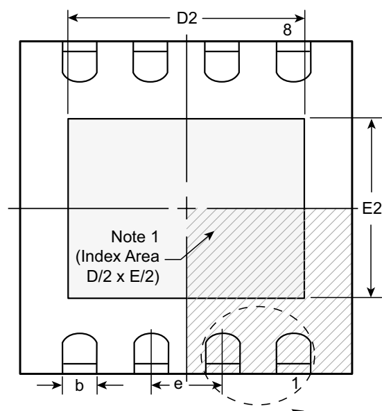
Bottom View
