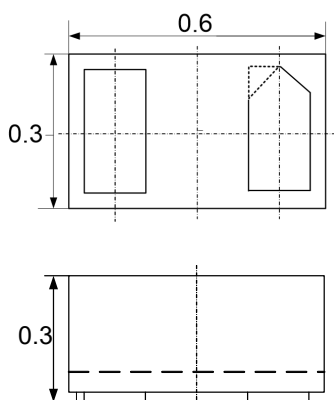
Package Dimensions
