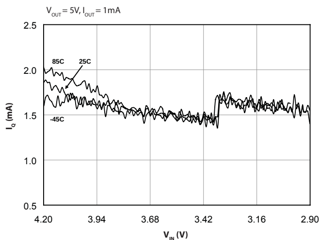
Quiescent Current
