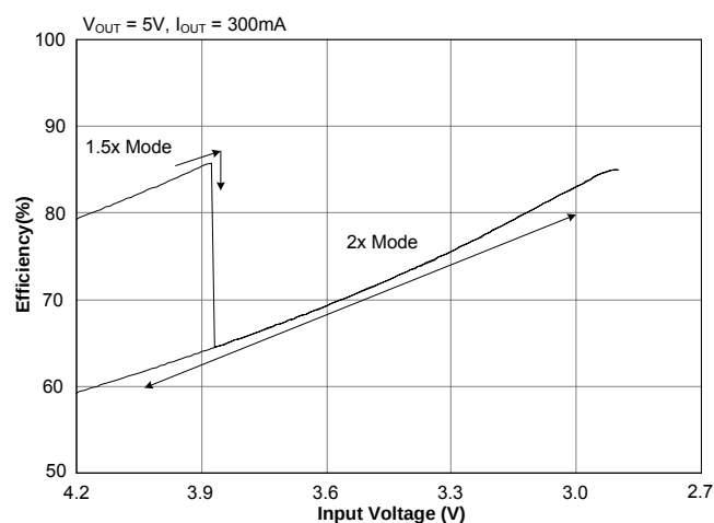
Efficiency — 300mA
