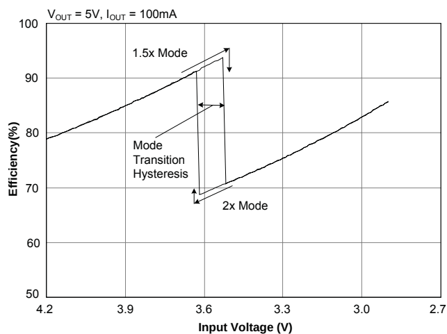
Efficiency — 100mA
