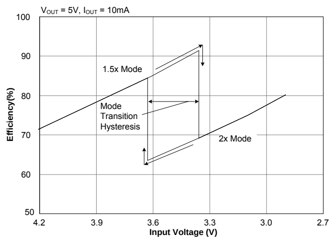
Efficiency — 10mA
