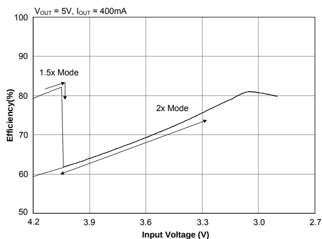
Efficiency — 400mA
