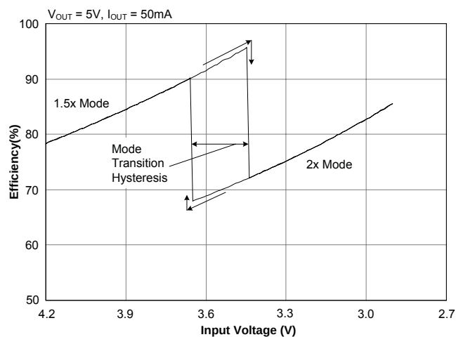
Efficiency — 50mA
