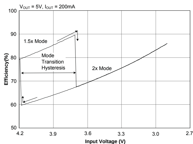
Efficiency — 200mA
