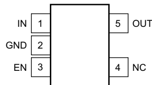
DBV Package 5-Pin SOT-23 Top View
