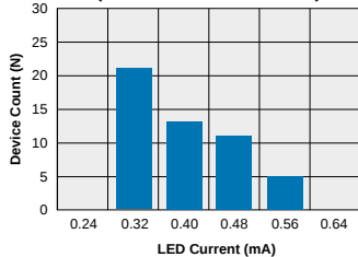
LBA120 - FormB Typical I_F for Switch Operation (N=50 Ambient Temperature = 25°C) (Load Current = 170mADC)
