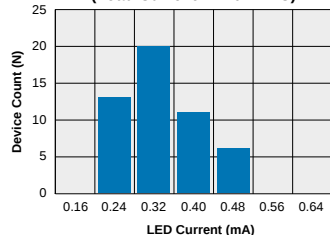
LBA120 - FormB Typical I_F for Switch Dropout (N=50 Ambient Temperature = 25°C) (Load Current = 170mADC)
