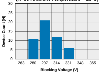
LBA120 - FormB Typical Blocking Voltage Distribution (N=50 Ambient Temperature = 25°C)
