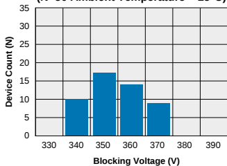
LBA120 - FormA Typical Blocking Voltage Distribution (N=50 Ambient Temperature = 25°C)
