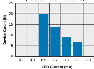
LBA120 - FormB Typical I_F for Switch Dropout (N=50 Ambient Temperature = 25°C) (Load Current = 170mADC)
