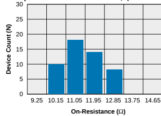
LBA120 - FormB Typical On-Resistance Distribution (N=50 Ambient Temperature = 25°C) (Load Current = 170mADC, I_F =5mADC)
