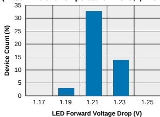
LBA120 Typical LED Forward Voltage Drop (N=50 Ambient Temperature = 25°C; I_F = 5mADC)
