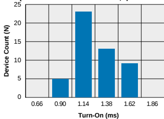
LBA120 - FormA Typical Turn-On Time (N=50 Ambient Temperature = 25°C) (Load Current = 170mADC; I_F = 5mADC)
