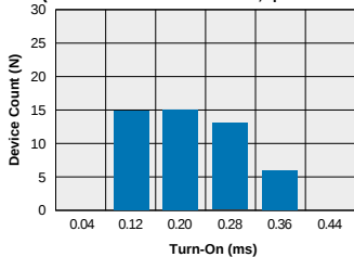
LBA120 - FormB Typical Turn-On Time (N=50 Ambient Temperature = 25°C) (Load Current = 170mADC; I_F = 5mADC)
