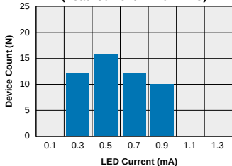
LBA120 - FormA Typical I_F for Switch Dropout (N=50 Ambient Temperature = 25°C) (Load Current = 170mADC)
