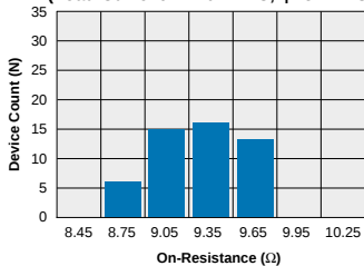
LBA120 - FormA Typical On-Resistance Distribution (N=50 Ambient Temperature = 25°C) (Load Current = 170mADC, I_F =5mADC)
