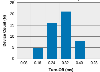
LBA120 - FormA Typical Turn-Off Time (N=50 Ambient Temperature = 25°C) (Load Current = 170mADC; I_F = 5mADC)
