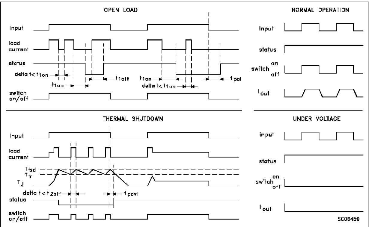
Figure 1: Waveforms
