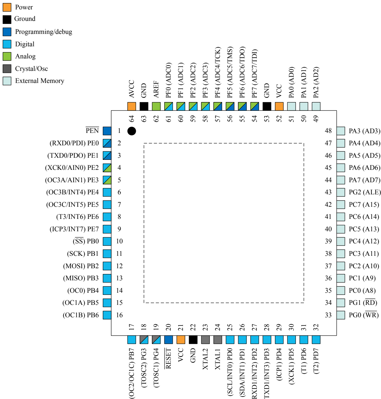
Figure 6-1 Pinout ATmega64A
