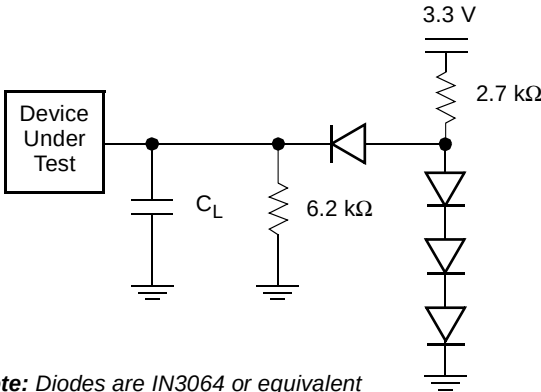
Figure 11. Test Setup
