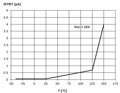
Figure 9: Standby current
