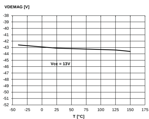
Figure 24: Turn-off output voltage clamp
