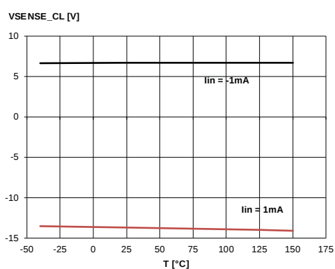
Figure 26: Vsense clamp vs. Tcase
