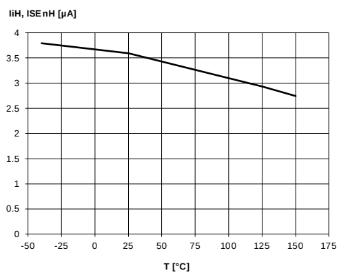
Figure 13: High level logic input current
