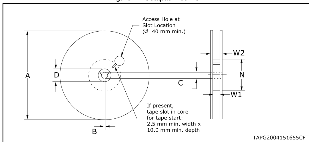
Figure 41: Octapak reel 13"
