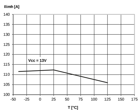
Figure 23: IlimH vs. Tcase
